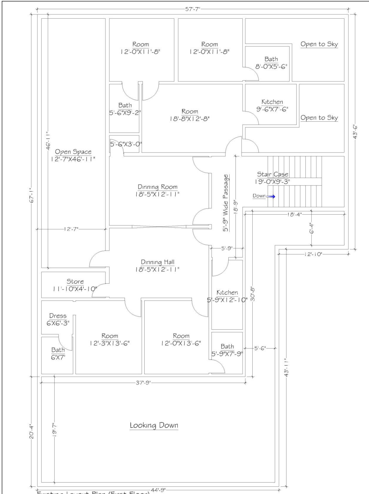
Existing Layout Plan (First Floor) Branch Code # Name: Kalat Branch Gawadar Region
