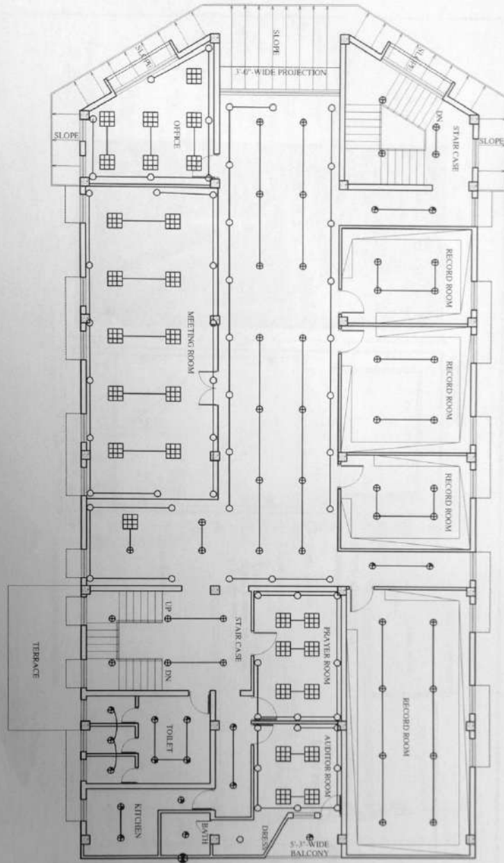
FIRST FLOOR ELECTRICAL POINTS WIRING PLAN
