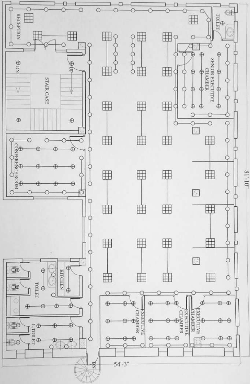
FIRST FLOOR ELECTRICAL POINTS WIRING PLAN
