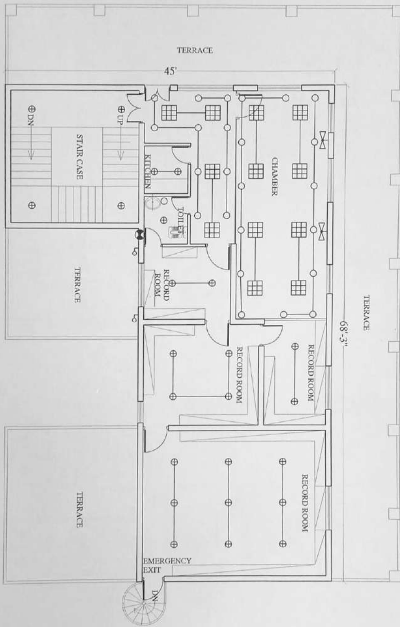
THIRD FLOOR ELECTRICAL POINTS WIRING PLAN
