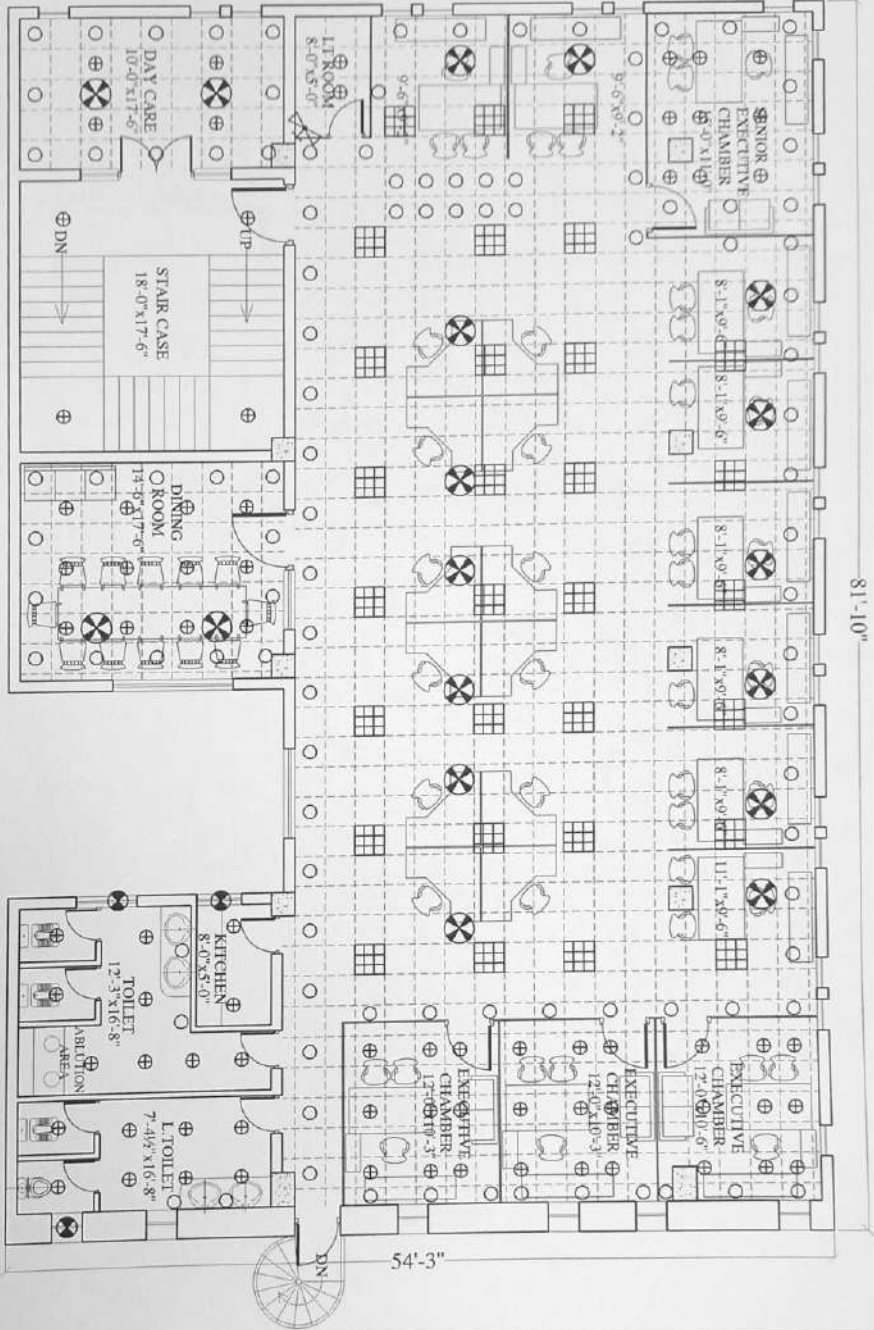
SECOND FLOOR ELECTRICAL LIGHTS & FANS PLAN COVERED AREA = 4190 Sft.
