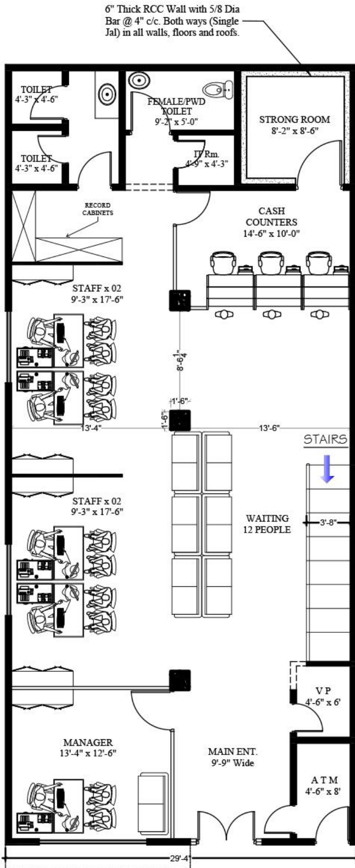
GROUND FLOOR (Proposed) Total Area = 1,945 SFT
