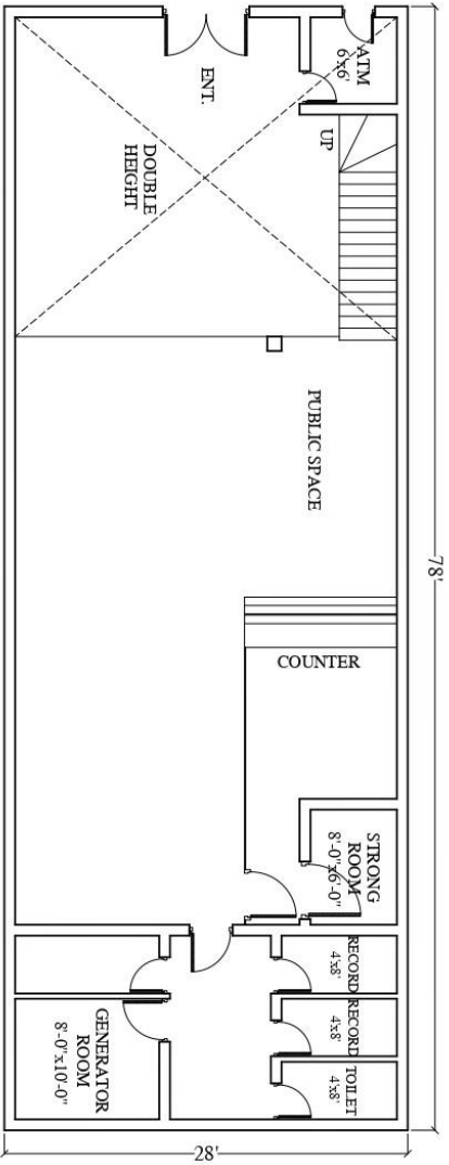
EXISTING GROUND FLOOR LAYOUT PLAN COVERED AREA = 2184 SF.
