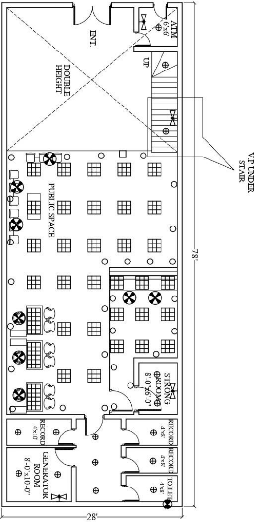
GROUND FLOOR ELECTRICAL LIGHTS & FANS PLAN COVERED AREA = 2184 SF.
