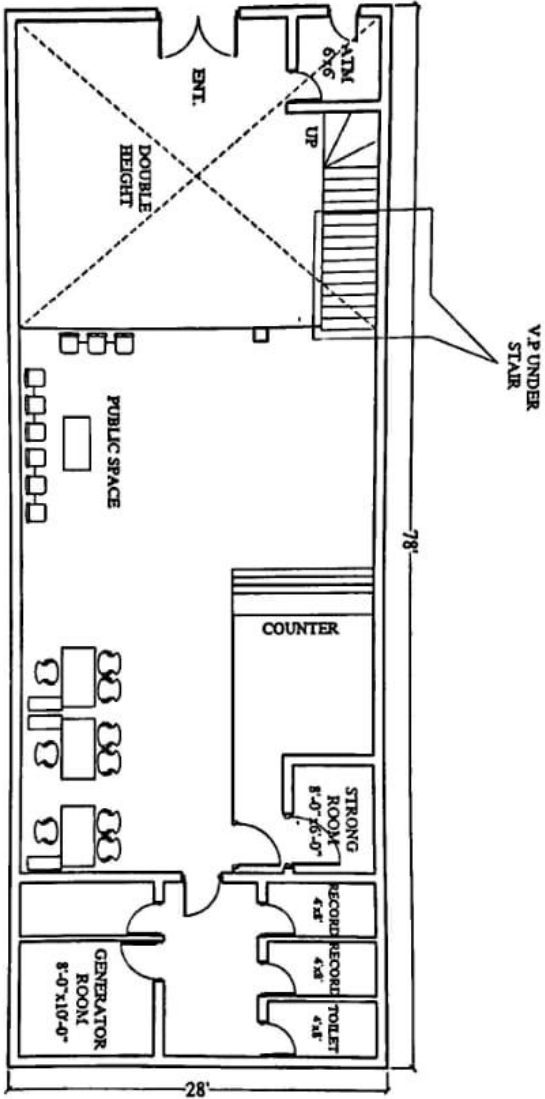
PROPOSED GROUND FLOOR LAYOUT PLAN COVERED AREA = 2184 SF.
