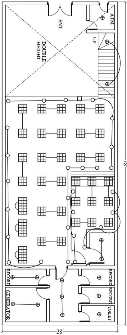
GROUND FLOOR ELECTRICAL POINTS WIRING PLAN
