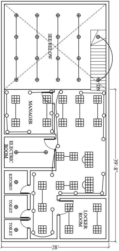
MEZZANINE FLOOR ELECTRICAL POINTS WIRING PLAN
