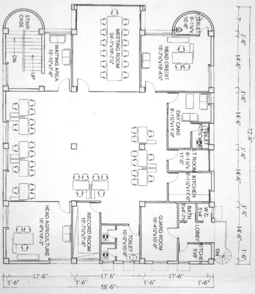
PROPOSED FIRST FLOOR LAYOUT PLAN COVERED AREA OF F.F. = 4139 Sq. Ft.
