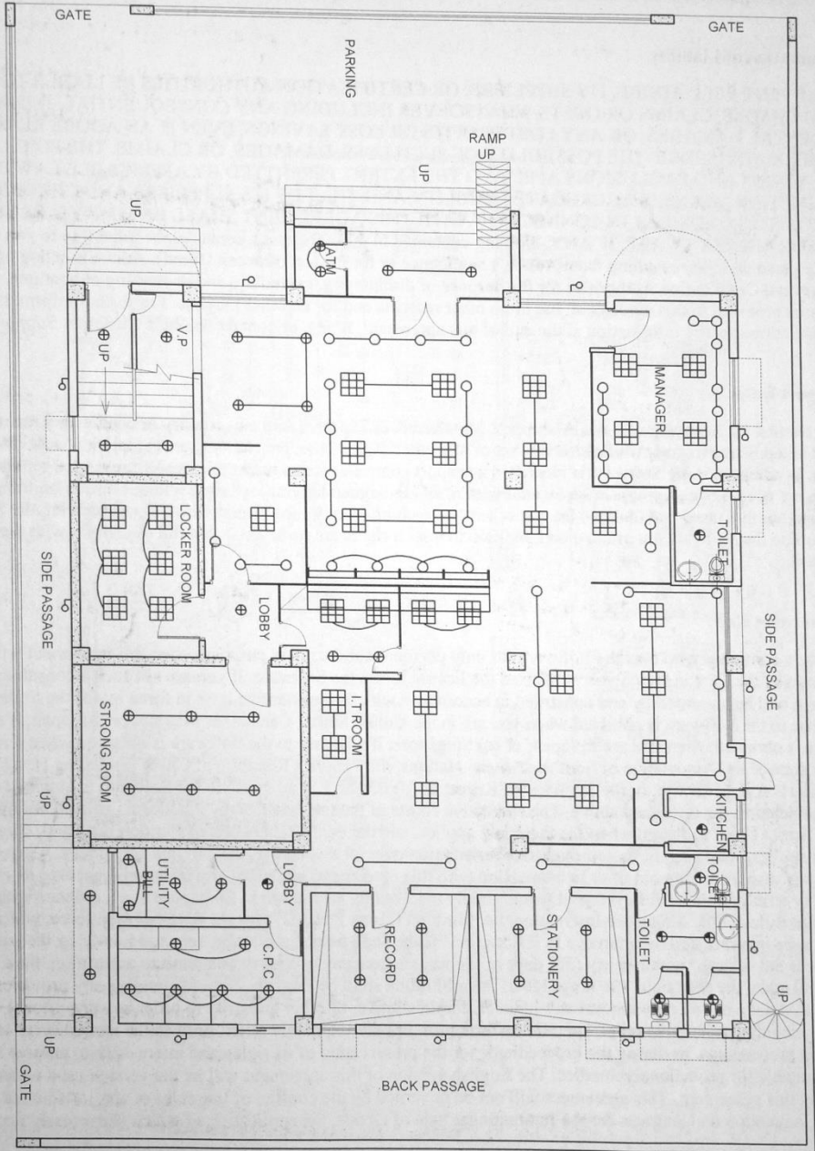
GROUND FLOOR ELECTRICAL POINTS WIRING PLAN
