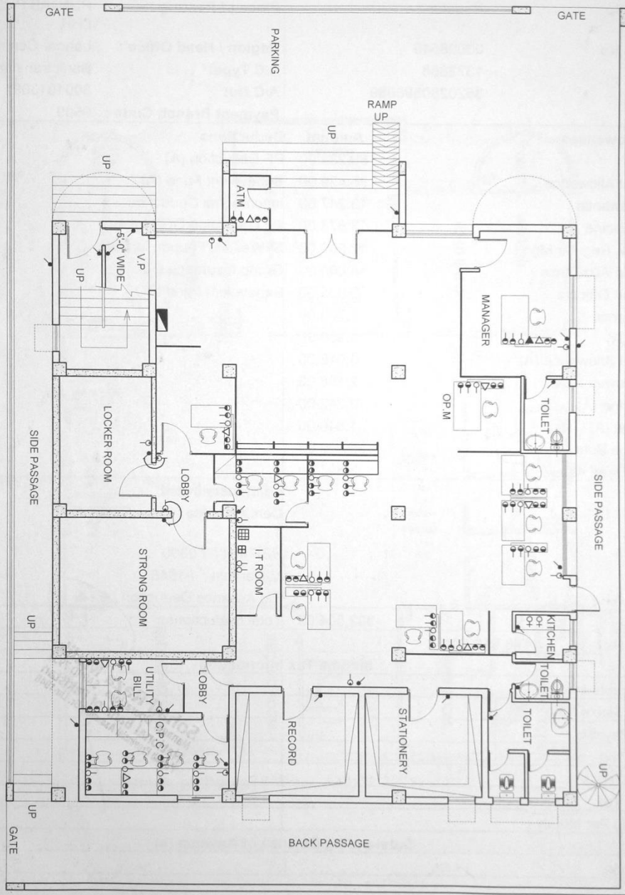
GROUND FLOOR ELECTRICAL PLAN FOR POWER, SOCKETS, TELEPHONE & LAN NODES
