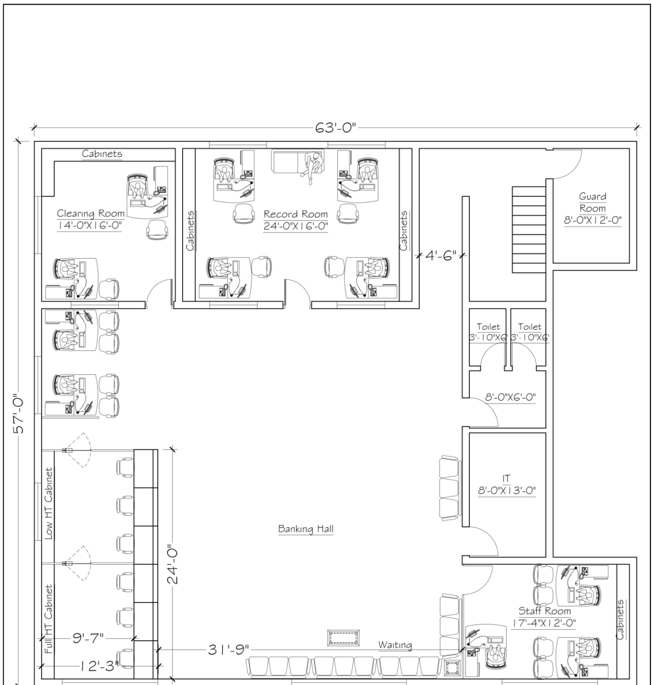
Proposed Layout Plan (First Floor) Branch Code # 0326 Name: Main Branch Dera Ghazi Khan DG Khan Region
