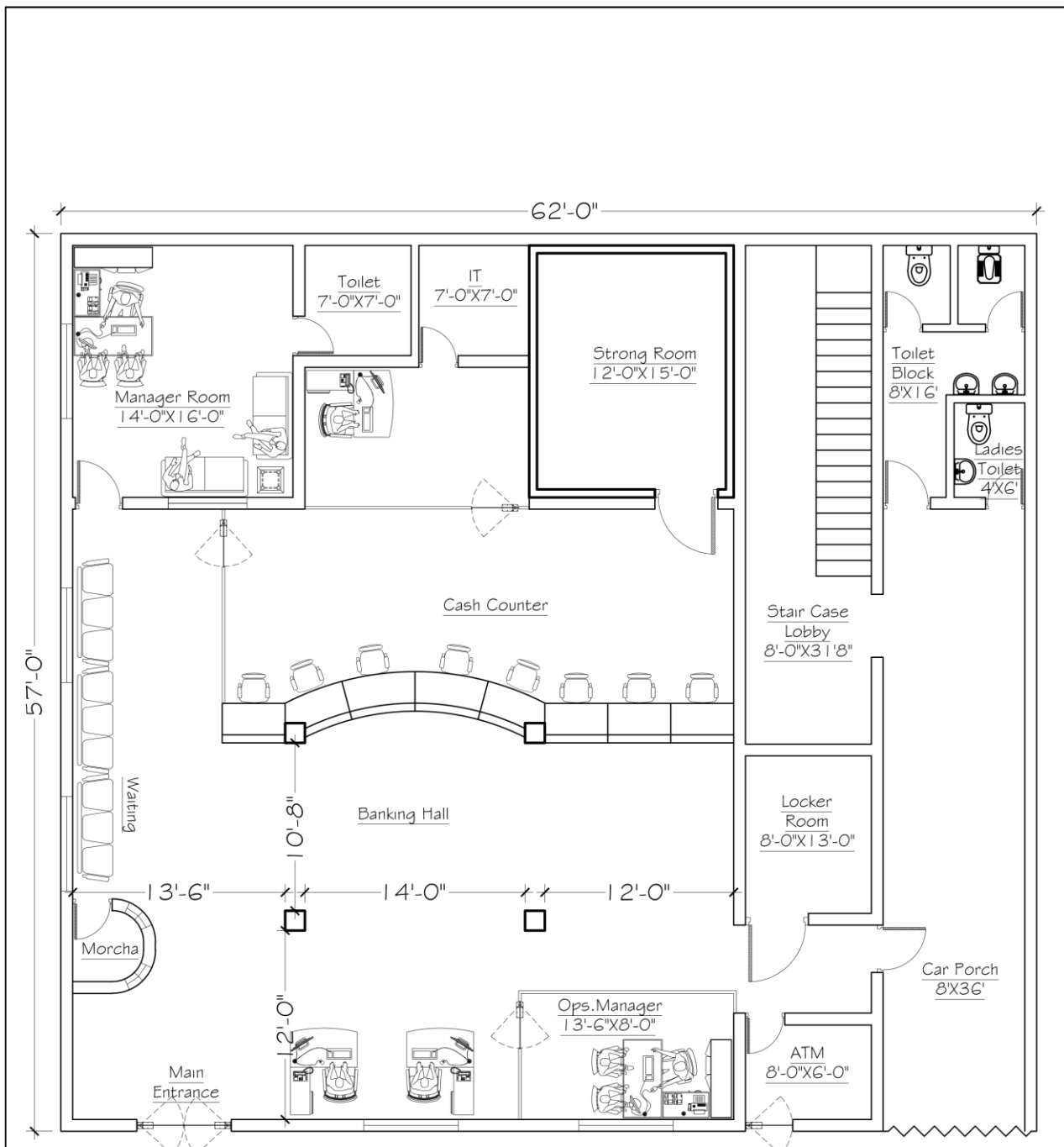
Existing Layout Plan (Ground Floor) Branch Code # 0326 Name: Main Branch Dera Ghazi Khan DG Khan Region
