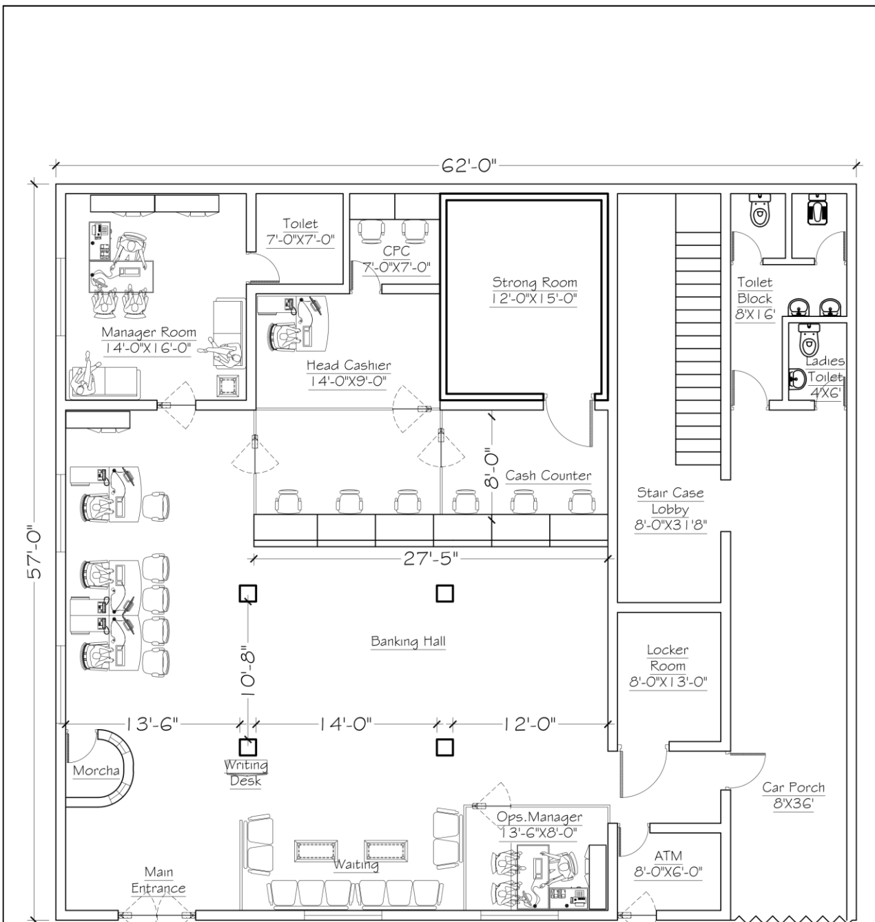
Proposed Layout Plan (Ground Floor) Branch Code # 0326 Name: Main Branch Dera Ghazi Khan DG Khan Region
