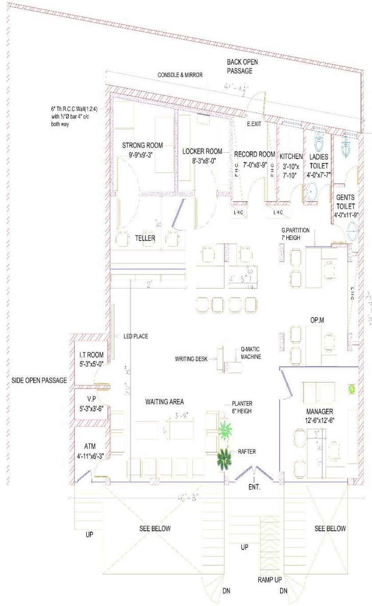
PROPOSED GROUND FLOOR LAYOUT PLAN
